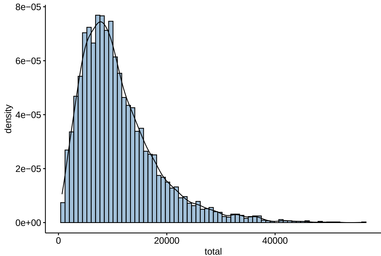
Cluster 7
